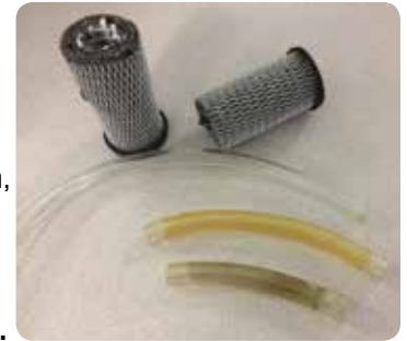
Cut Filter & Hoses show Improper Maintenance & Bacteria Growth.
